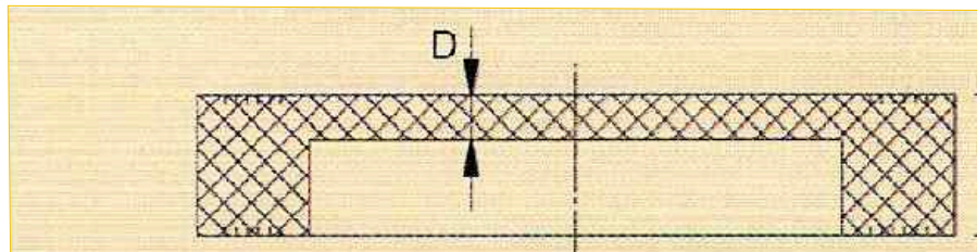
Bursting Disc with Support Grill
