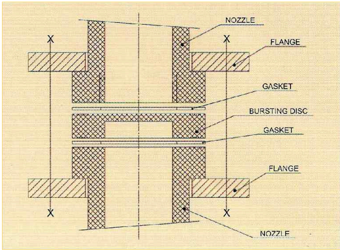
Bursting Disc
